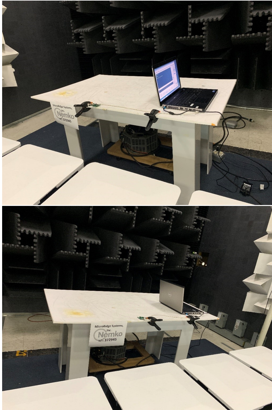
Figure 8.1-2: Clause 9.2 – Radio frequency electromagnetic field (2.7 GHz to 6GHz) setup photo
